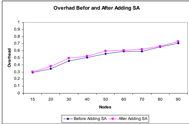
Figure 7: Overhead before and after adding SA to CBRP
